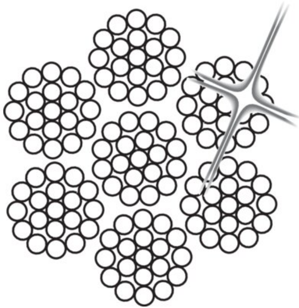
Winch rope
