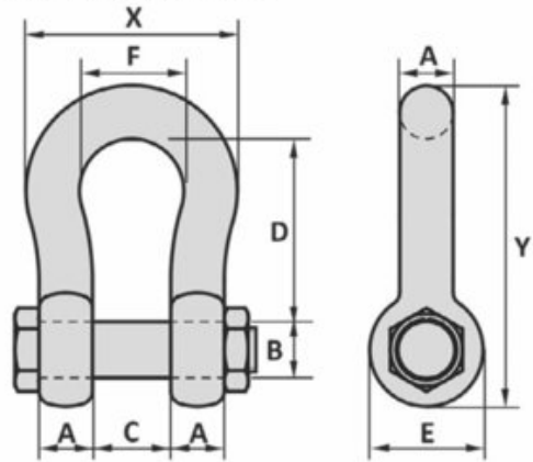
BOW TYPE SAFETY PIN
